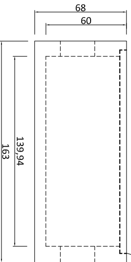
VISTA FRONTAL
